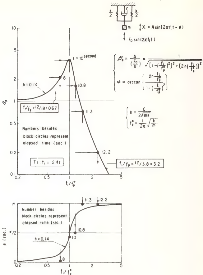
Fig. 12 Estimation of Apparent Natural Frequency of Pile Foundation Model Embedded in Liqueifying Sand Layer (Test 1)
